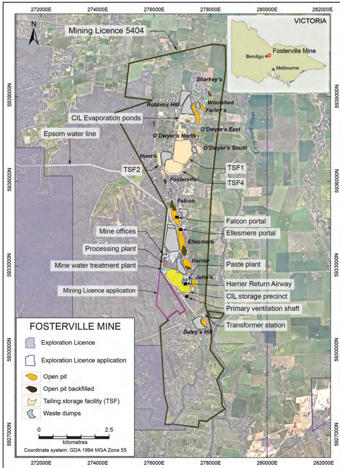
Surface Plan of the Fosterville mine (as at December 31, 2022)
