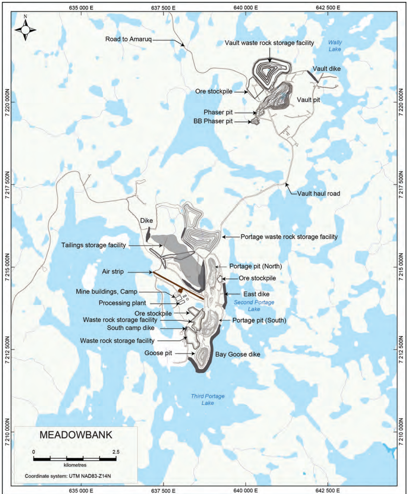
Surface Plan of the Meadowbank Mine (as at December 31, 2022)
